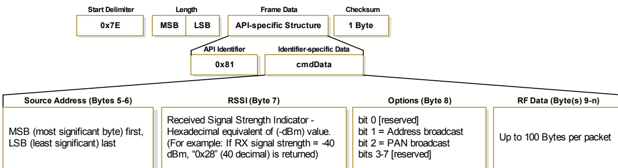
Figure 26: RX Packet (16-bit address) frames
